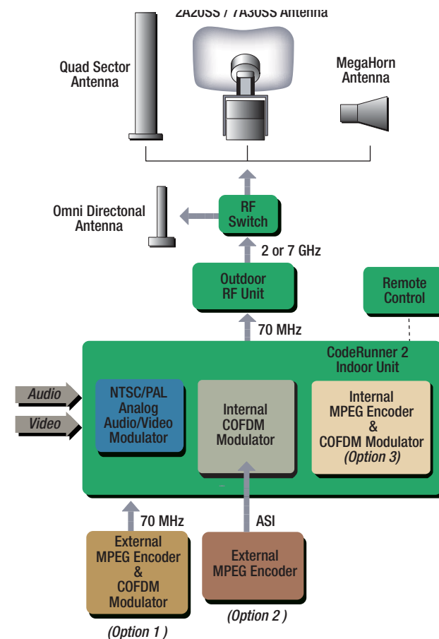
CodeRunner 2 upgrade options using internal and external modulators and encoders.
